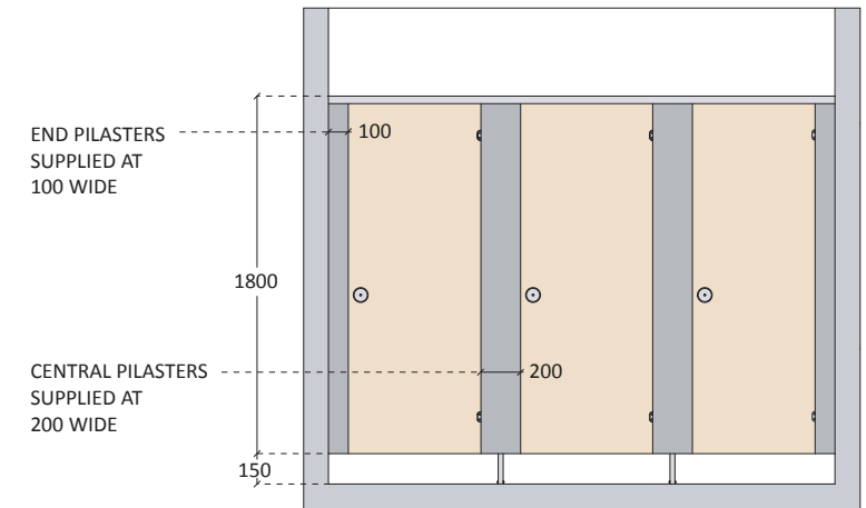
Typical Front Elevation
